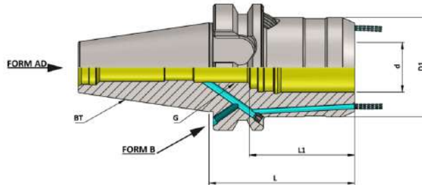
BT (MAS 403) Hydraulic Expansion Chuck (FCC - AD+B)
