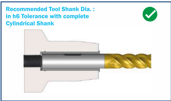
CLAMPING WITH RS SLEEVE
