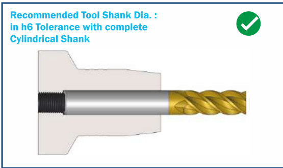
DIRECT CLAMPING
