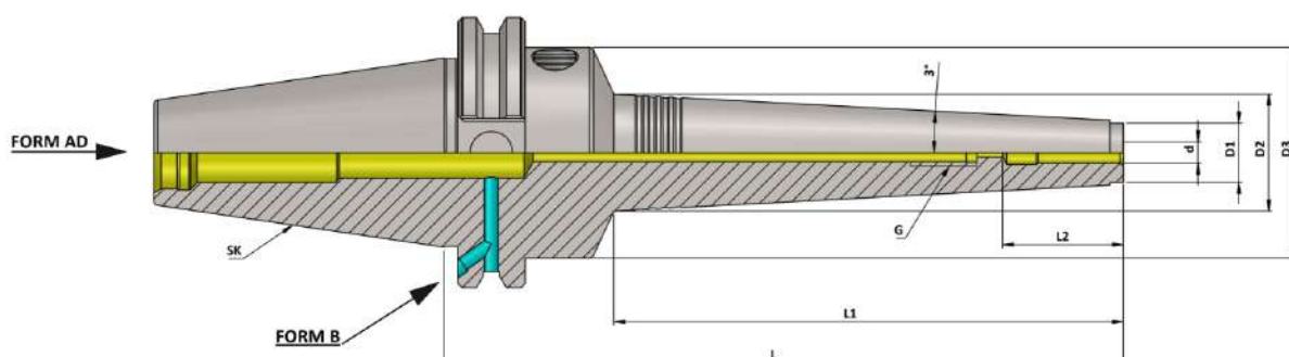
SK(DIN 69871) Hydraulic Expansion Chuck Slim 3 Degree (AD+B) (AD/AF)
